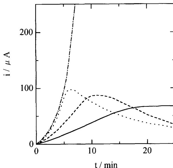
Fig. 1. Potentiostatic current transient for film deposition from 0.1 M aniline solutions of different PSS fractions ( -\text{SO}_3^-/(-\text{SO}_3^- + \text{Cl}^-) ) (—) 1, (---) 0.5, (·····) 0.1, and (– · – · –) 0. Electrode potentials were stepped from the rest potential to 0.8 V.
