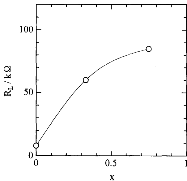
Fig. 10. Plots of the Warburg-region width R_L against the PSS fraction x for films having a Q_{0.4} value of 3.1 \text{mC cm}^{-2} . Electrolyte solution: 0.3 M (HPSS+HCl). Applied potential: -0.1 V.
