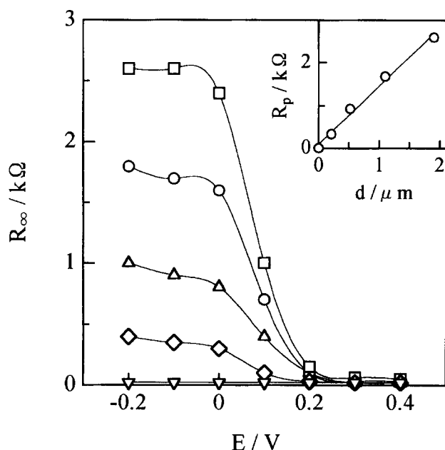
Fig. 5. Plots of high-frequency resistance R_\infty against applied potential at different film thicknesses (▽) 0, (◇) 0.21, (△) 0.52, (○) 1.1, and (□) 1.9 \mu\text{m} . Electrolyte solution: 0.5 M HPSS. The inset shows a linear increase in the film resistance at -0.1 V with increasing film thickness.
