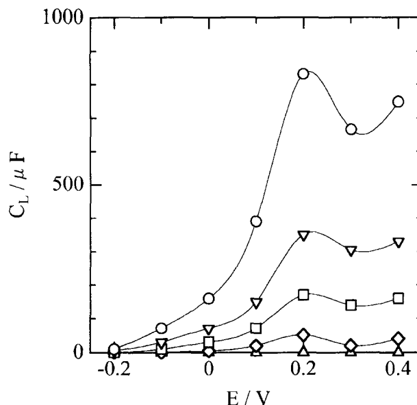
Fig. 7. Low-frequency capacitance versus applied potential plots at different film thicknesses ( \Delta ) 0, ( \diamond ) 0.21, ( \square ) 0.52, ( \nabla ) 1.1, and ( \circ ) 1.9 \mu\text{m} . Electrolyte solution: 0.3 M HCl.
