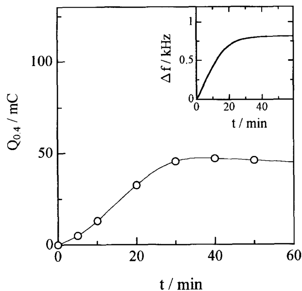
Fig. 2. The charge for the first redox process, Q_{0.4} , measured at different stages of electrodeposition. A PA/PSS film was deposited at 0.8 V from a 0.1 M solution of aniline in 0.5 M HPSS. The inset shows the EQCM frequency response for a PA/PSS-modified electrode held at 0.8 V in aniline-free 0.1 M \text{HClO}_4 .
